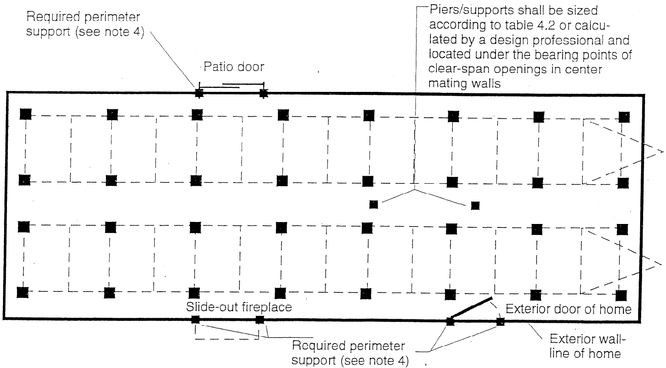
Figure 4-3 -- Typical blocking diagram for multisection home when manufacturer's installation instructions are not available
