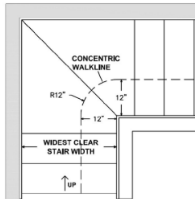
FIGURE R311.7.4 WINDER TREAD AND LANDING DETAIL
