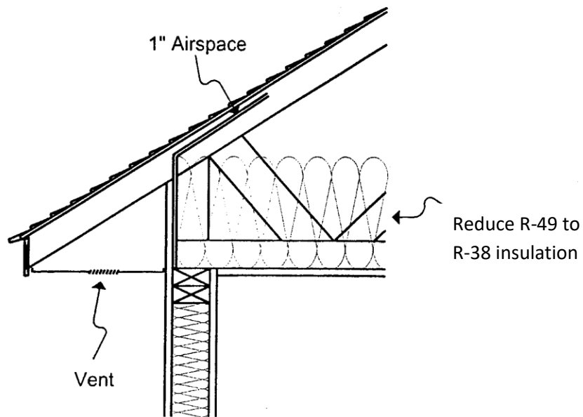
Fig. 2: Raised-Heel Truss
