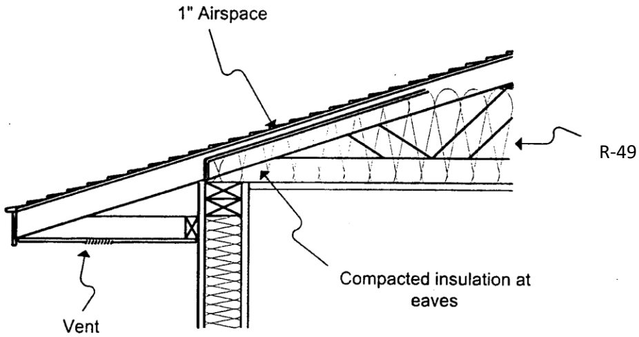
Fig. 1: Typical Insulation Practice on Low-Slope Roofs
