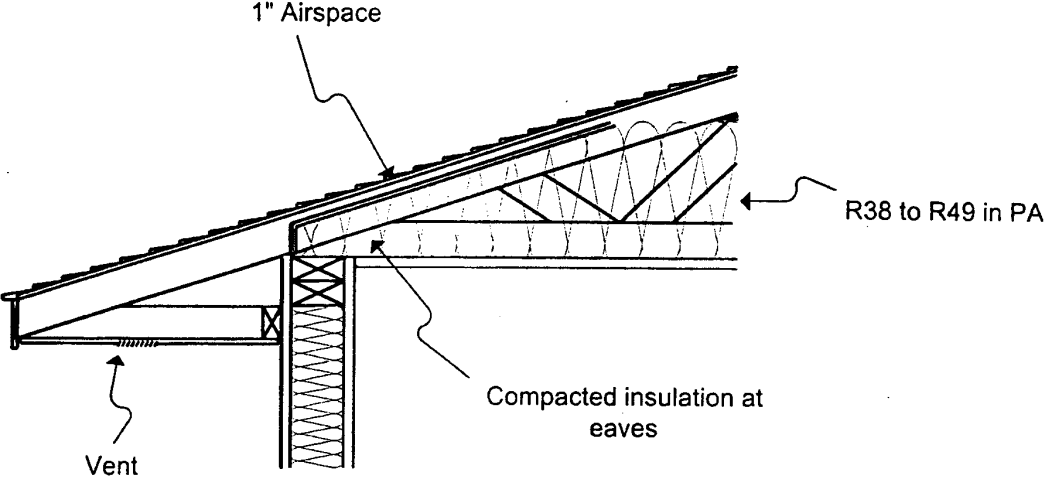
Fig. 1: Typical Insulation Practice on Low-Slope Roofs
