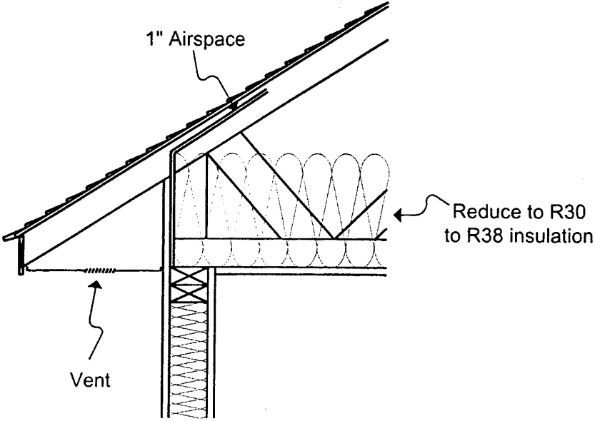
Fig. 2: Raised-Heal Truss
